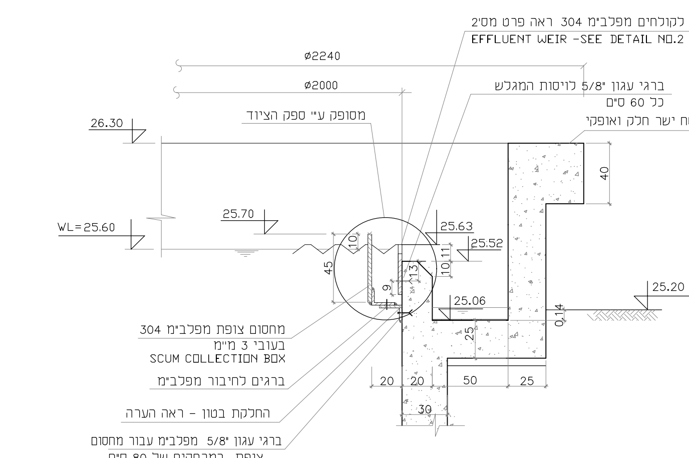
DETAIL NO.2: EFFLUENT WEIR 1:10
