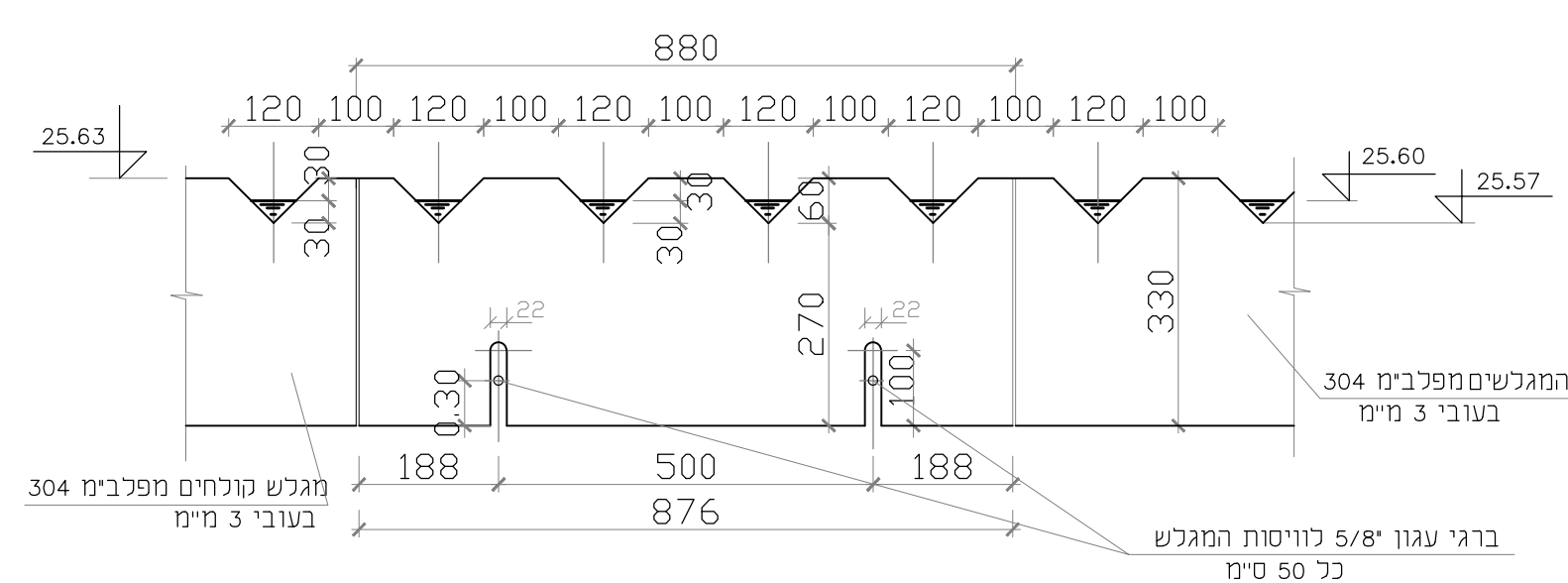
DETAIL NO.2: EFFLUENT WEIR 1:10
